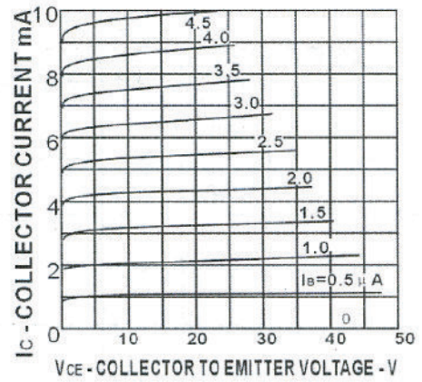
FIG.2 Collector Current vs Collector to Emitter Voltage
